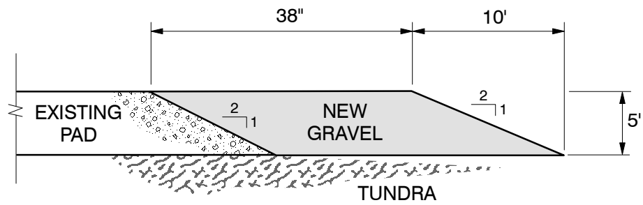
GRAVEL CROSS SECTION A - A'
